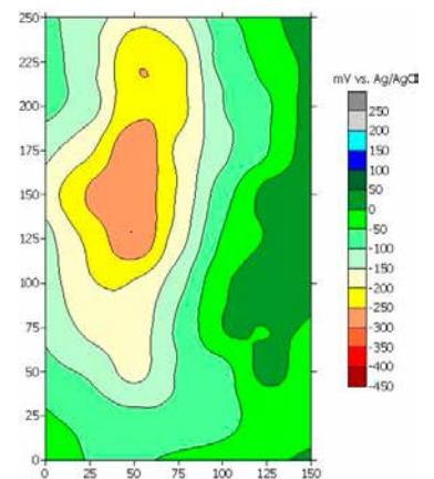
Contour plot from measurements carried out on the concrete deck in swimming pool
