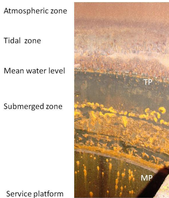
FIGURE 5: Appearance of corroded surface inside a monopile.
