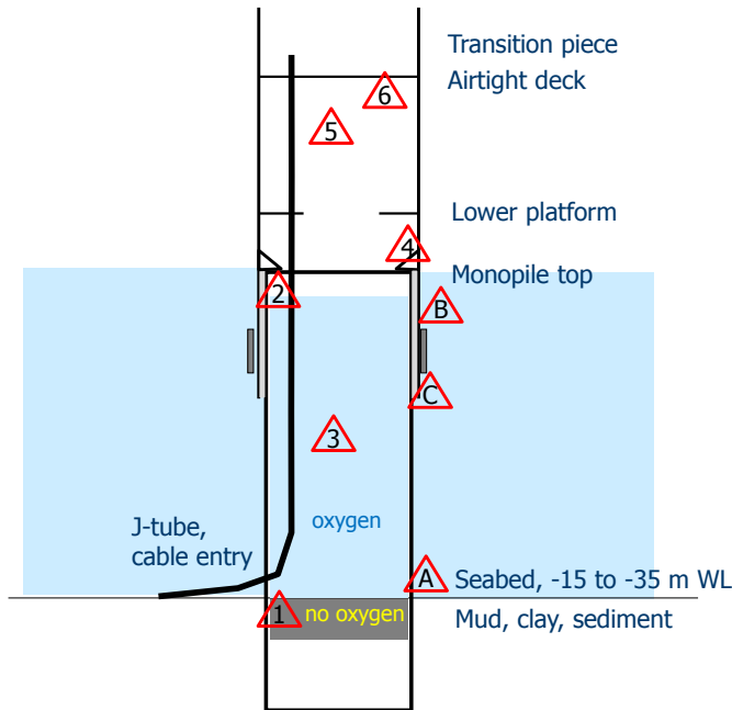
FIGURE 1: Risks related to corrosion in the monopile foundation design.
