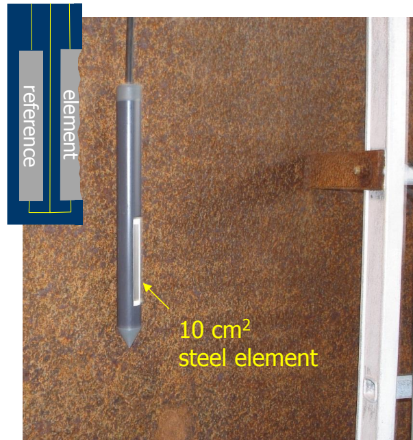
FIGURE 15: Principle and photo of ER-probe used for real-time corrosion rate measurement inside a monopile.
