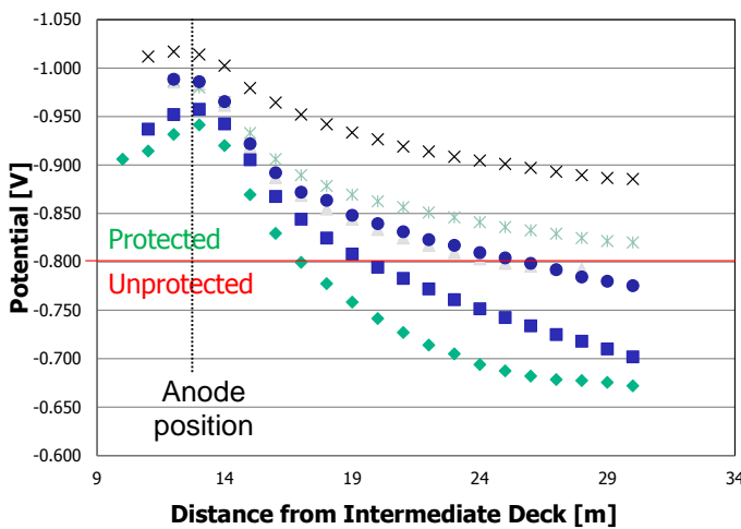
FIGURE 11: Example of drop-cell measurements obtained in a wind farm, where some of the foundations initially were under-protected.
