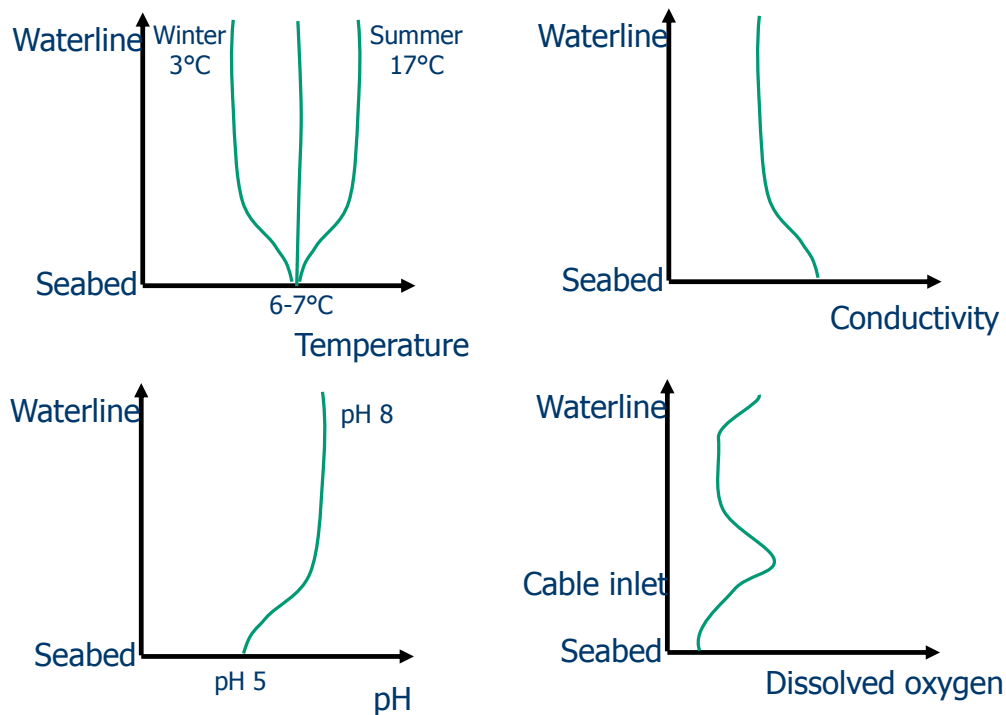
FIGURE 13: Trends observed using a drop-cell rack for environmental monitoring inside monopiles.
