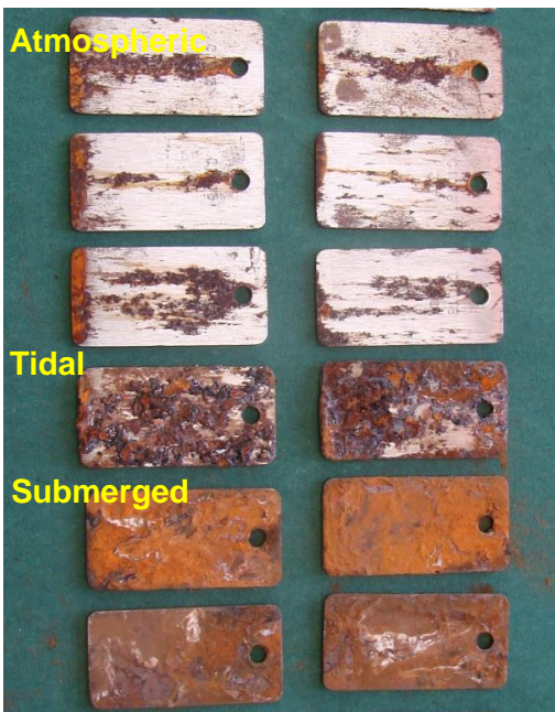
FIGURE 9: Corrosion coupons exposed inside monopile in three different corrosion zones.
