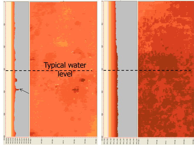
FIGURE 8: Results obtained with UT-crawler in two positions at the waterline. A maximum pit depth of 2.8 mm is observed on the inside in the left scan.
