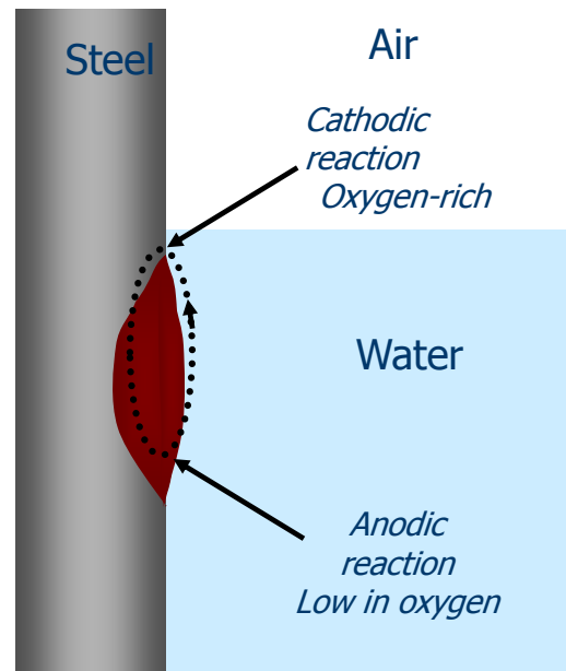
FIGURE 2: Example of localized corrosion mechanism at the waterline inside the monopile.
